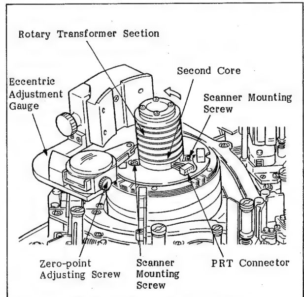
Fig. 6-5-1 Eccentric Adjustment
